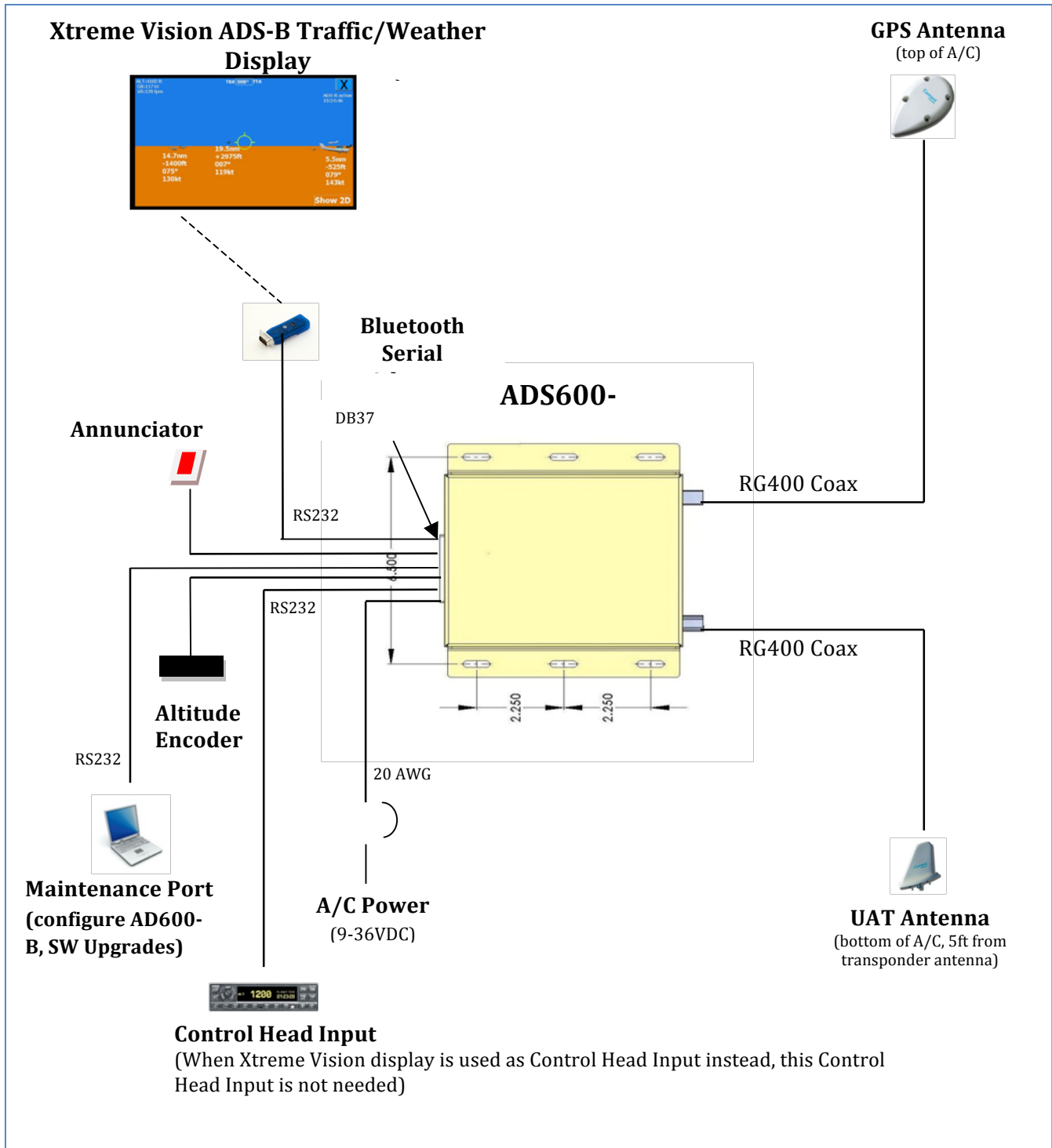
ADS600-B™ and Xtreme Vision display of ADS-B Traffic and Weather
