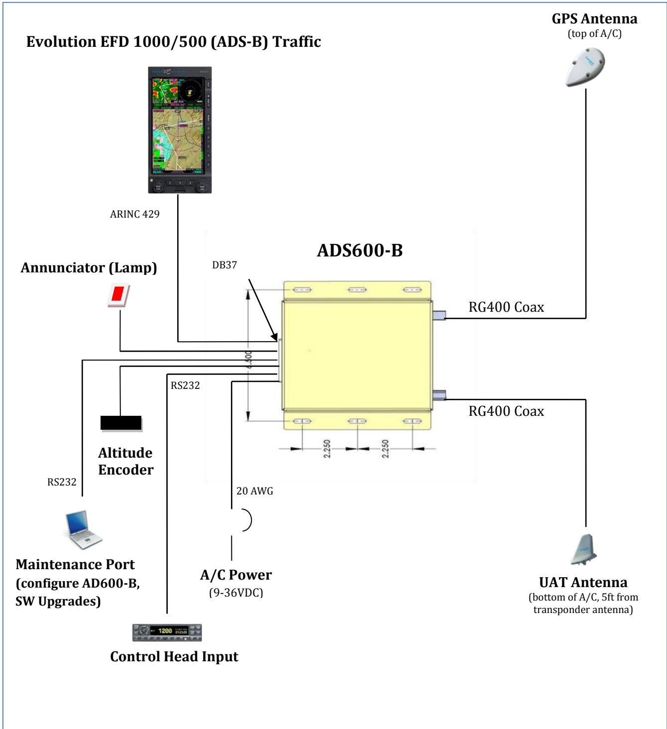
ADS600-B™ and Evolution EFD 1000/500 display of ADS-B Traffic
