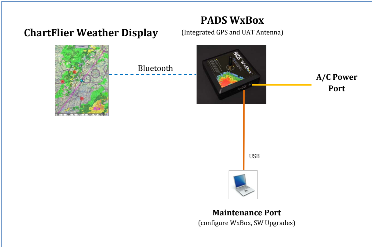
PADS® WxBox™ and Chartflier display of ADS-B Weather
