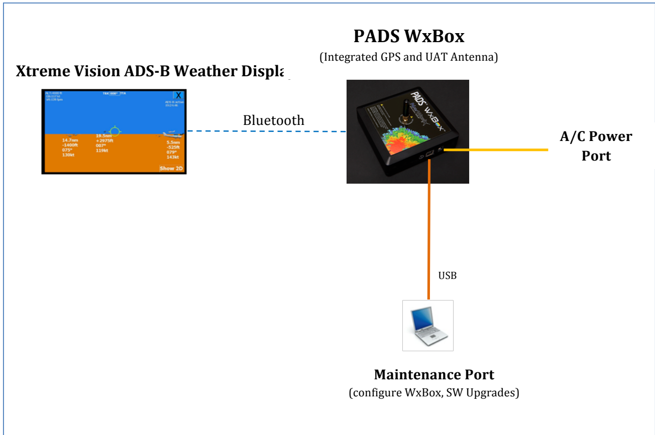
PADS® WxBox™ and Xtreme Vision display of ADS-B Weather
